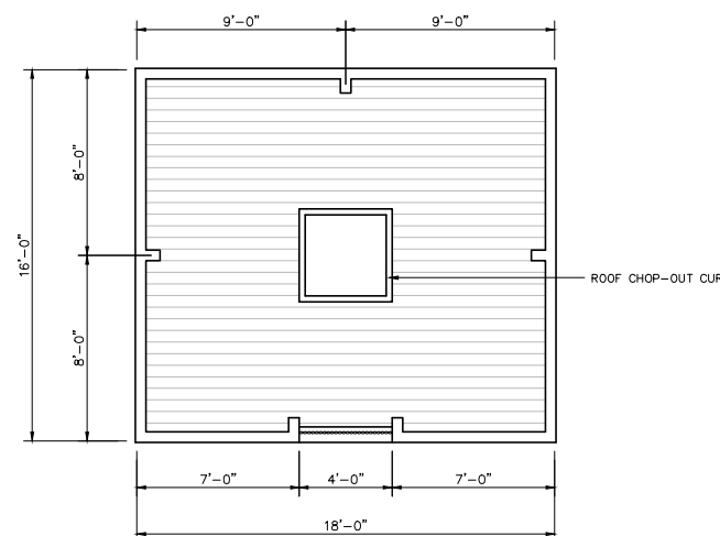
ROOF PLAN
